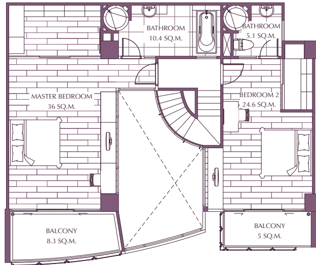
UPPER FLOOR
